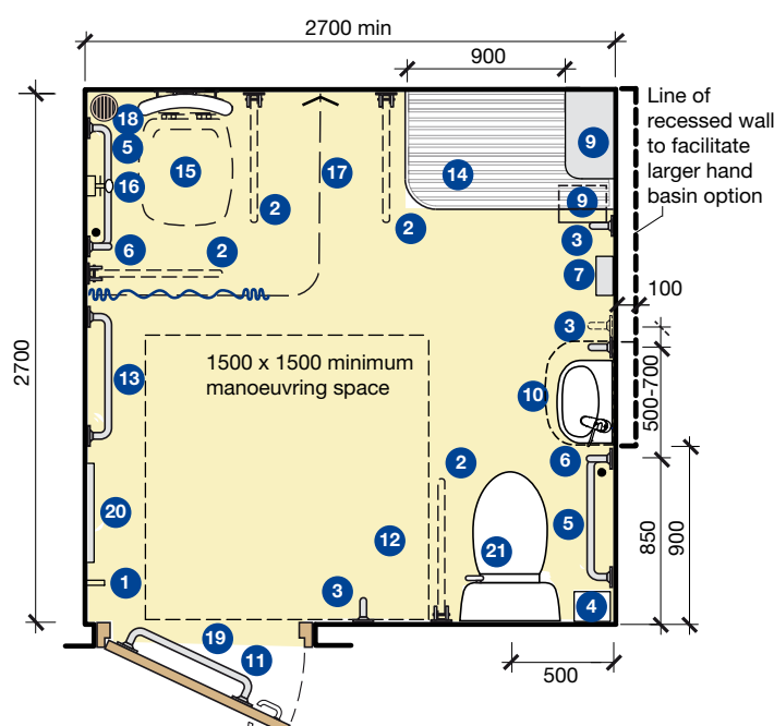
Figure 16 Unisex Accessible Changing Room
