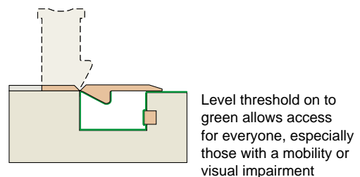
Figure 30 Typical sections through side or end ditch
