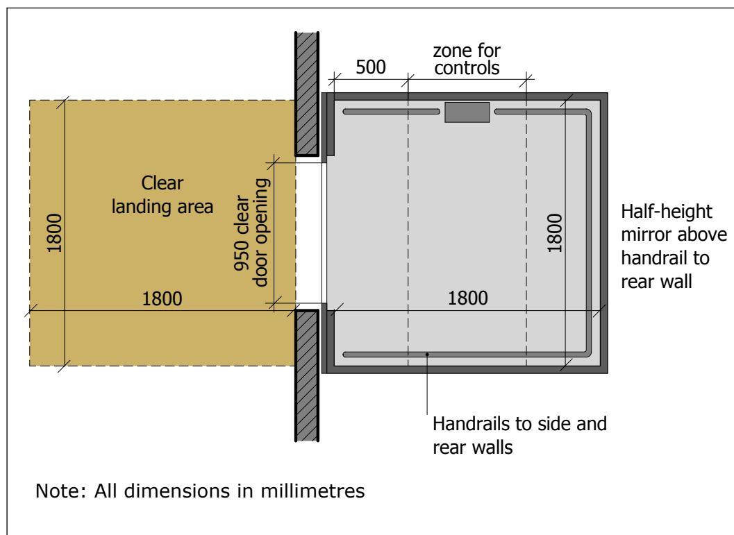
Figure 3.6 Passenger lift.
