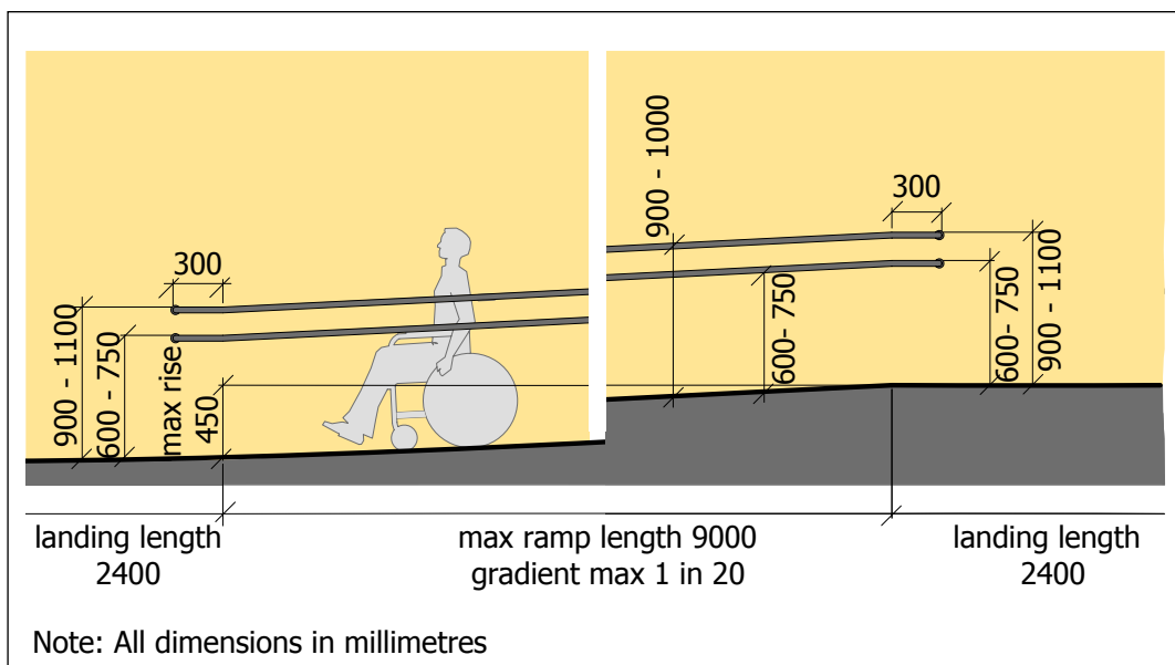
Figure 3.4 Internal ramp.
