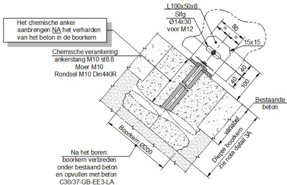
Figuur 32-34-7: Detail 3B – verankering in beton
