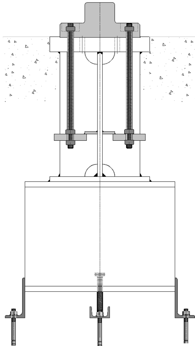
Figuur 32-11-3: railsysteem 3
